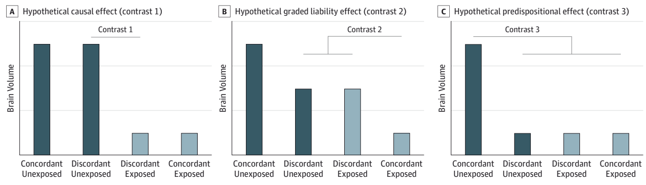
Figure 1. Hypothetical Causal and Predispositional Effects
