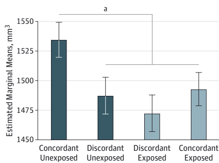
Figure 2. Left Amygdala Volume by Cannabis Exposure Group
